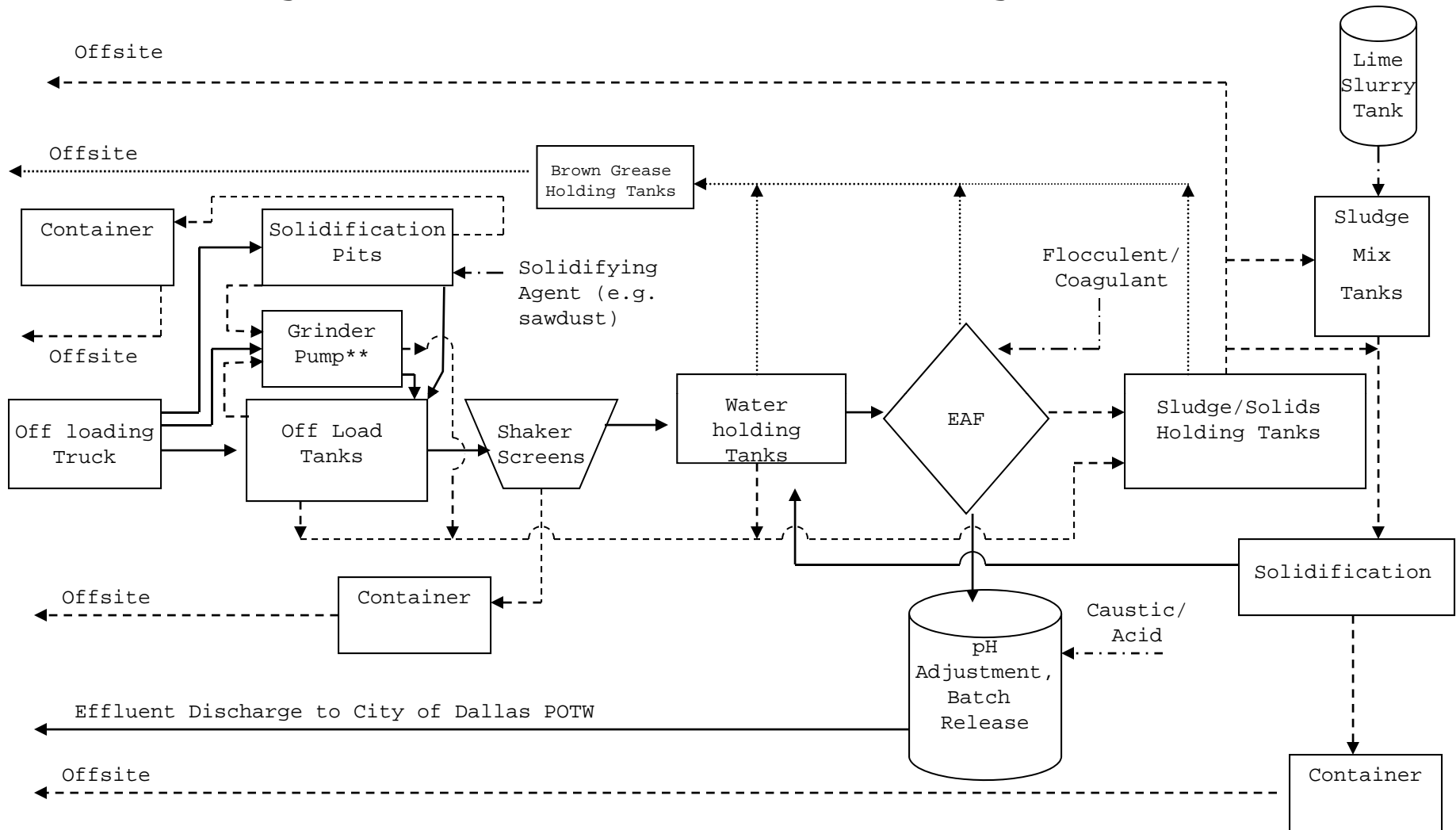
Liquid Environmental Solutions Figure SDP-1: Grease Process Flow Diagram
