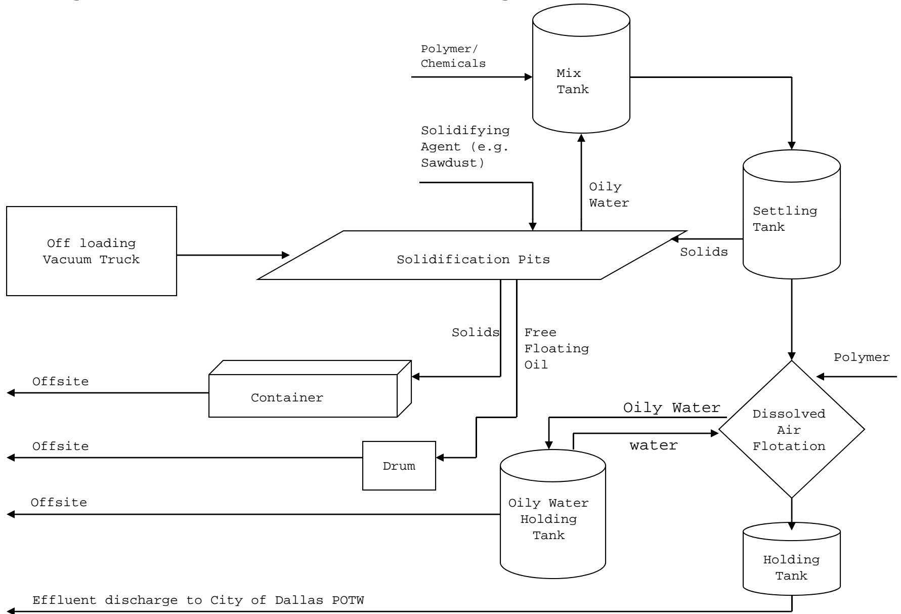
Liquid Environmental Solutions Figure SDP-2: Grit Process Flow Diagram
